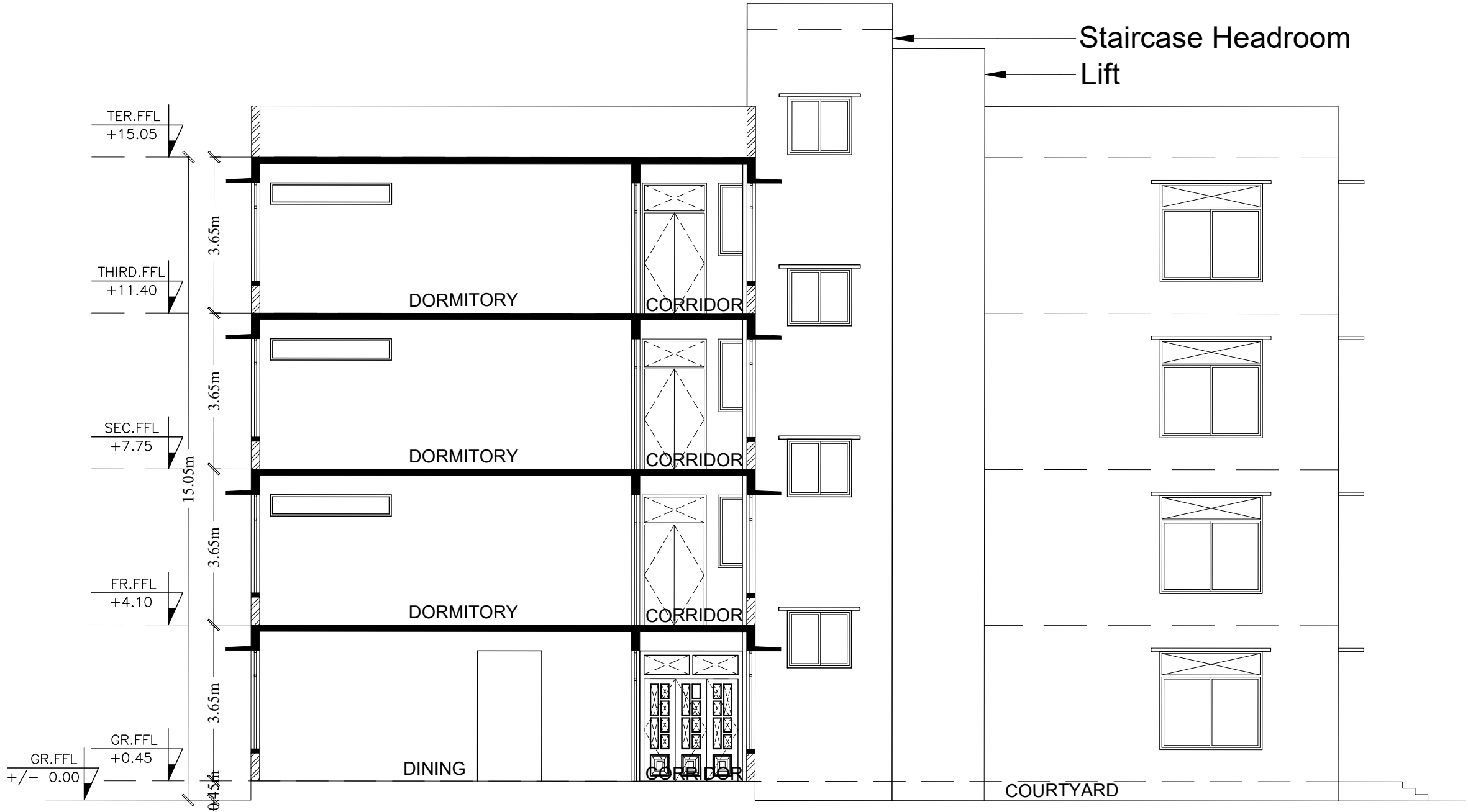
SECTION AT A-A
